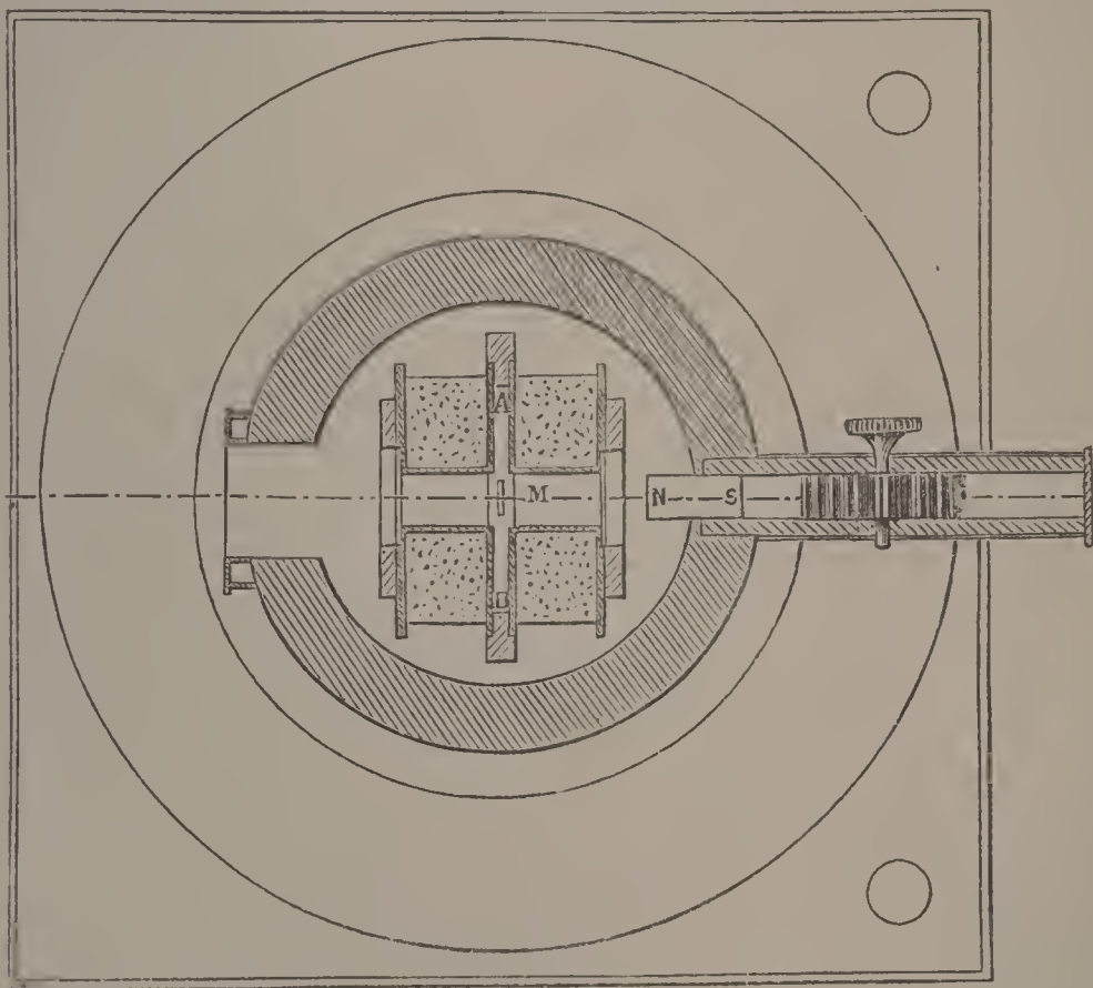
Sectional Plan.
